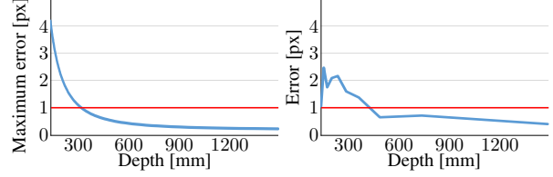
(a) Maximum approximation error (b) Error against Zemax
